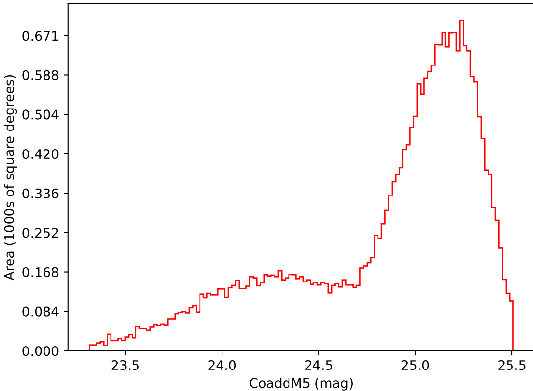
retro_baseline_v2.0_10yrs Yr 1 i band: CoaddM5
