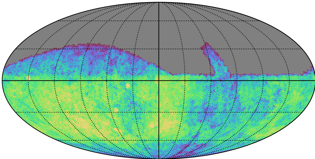
retro_baseline_v2.0_10yrs Yr 1 g band: CoaddM5
