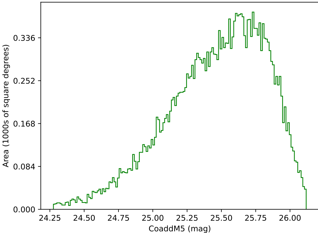
retro_baseline_v2.0_10yrs Yr 1 g band: CoaddM5
