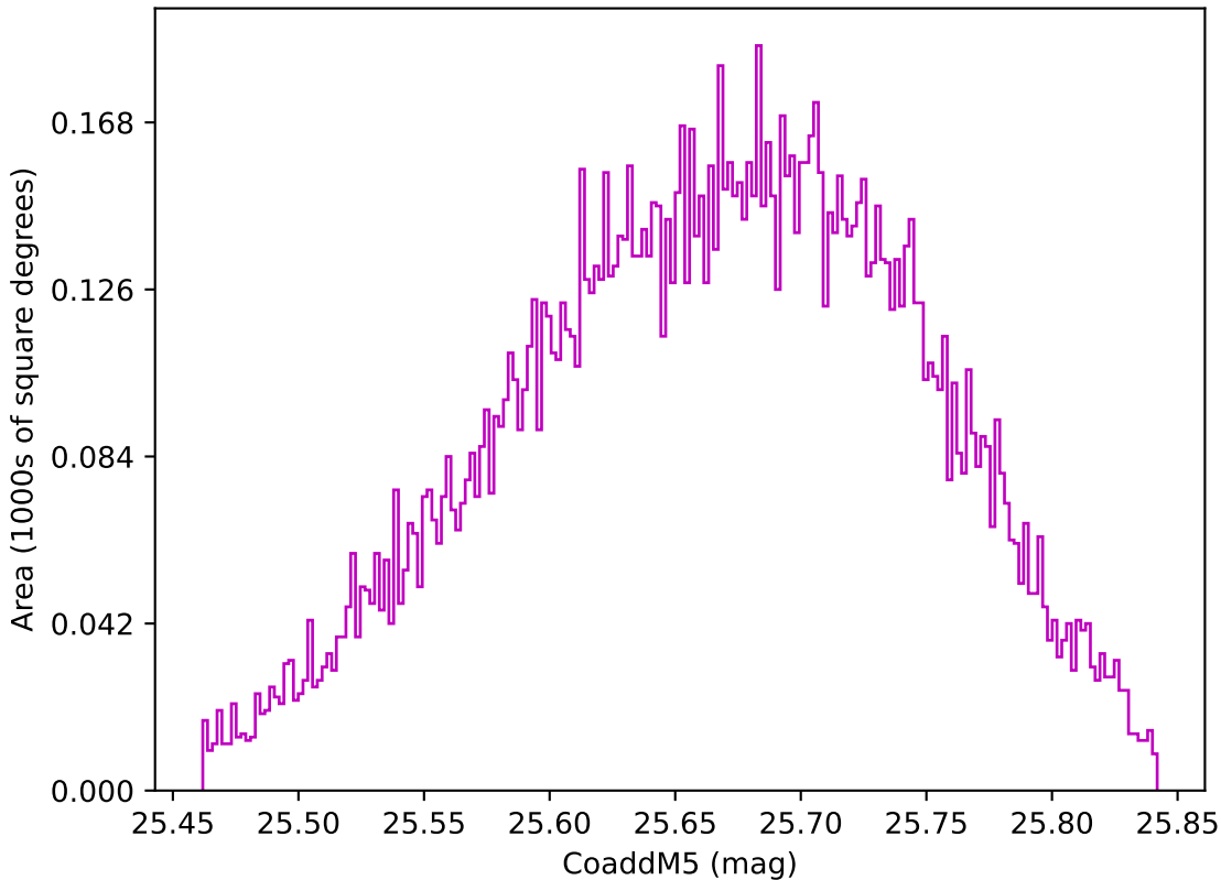
retro_baseline_v2.0_10yrs WFD z band: CoaddM5
