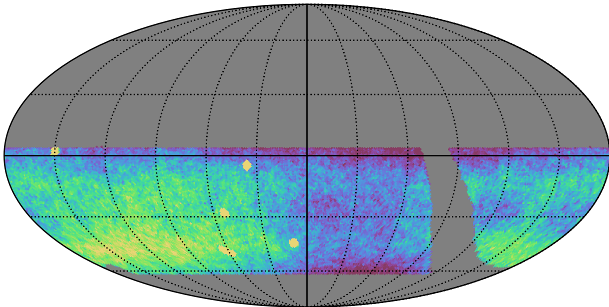
retro_baseline_v2.0_10yrs WFD y band: CoaddM5
