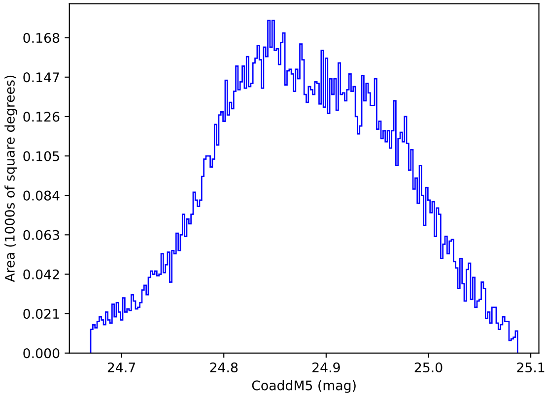
retro_baseline_v2.0_10yrs WFD y band: CoaddM5
