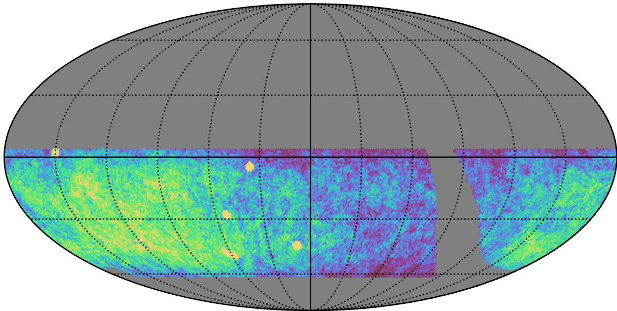
retro_baseline_v2.0_10yrs WFD u band: CoaddM5
