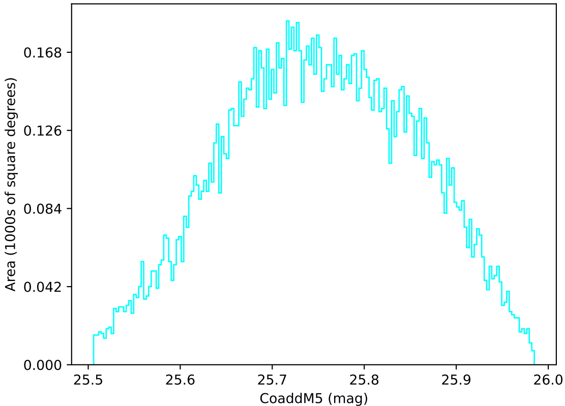
retro_baseline_v2.0_10yrs WFD u band: CoaddM5
