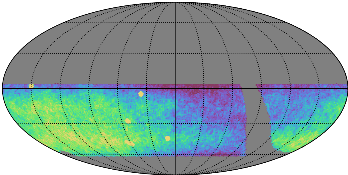
retro_baseline_v2.0_10yrs WFD r band: CoaddM5
