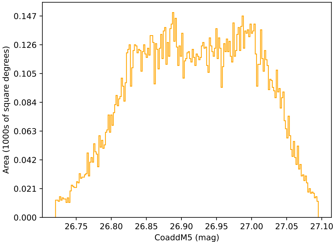
retro_baseline_v2.0_10yrs WFD r band: CoaddM5
