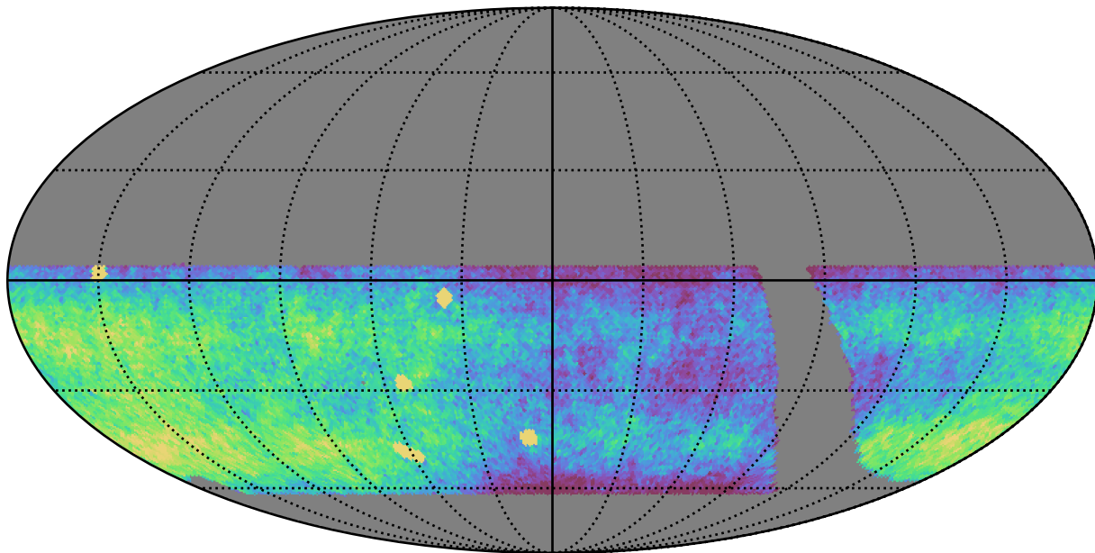
retro_baseline_v2.0_10yrs WFD i band: CoaddM5
