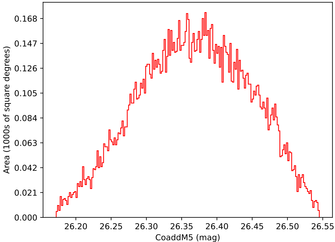
retro_baseline_v2.0_10yrs WFD i band: CoaddM5
