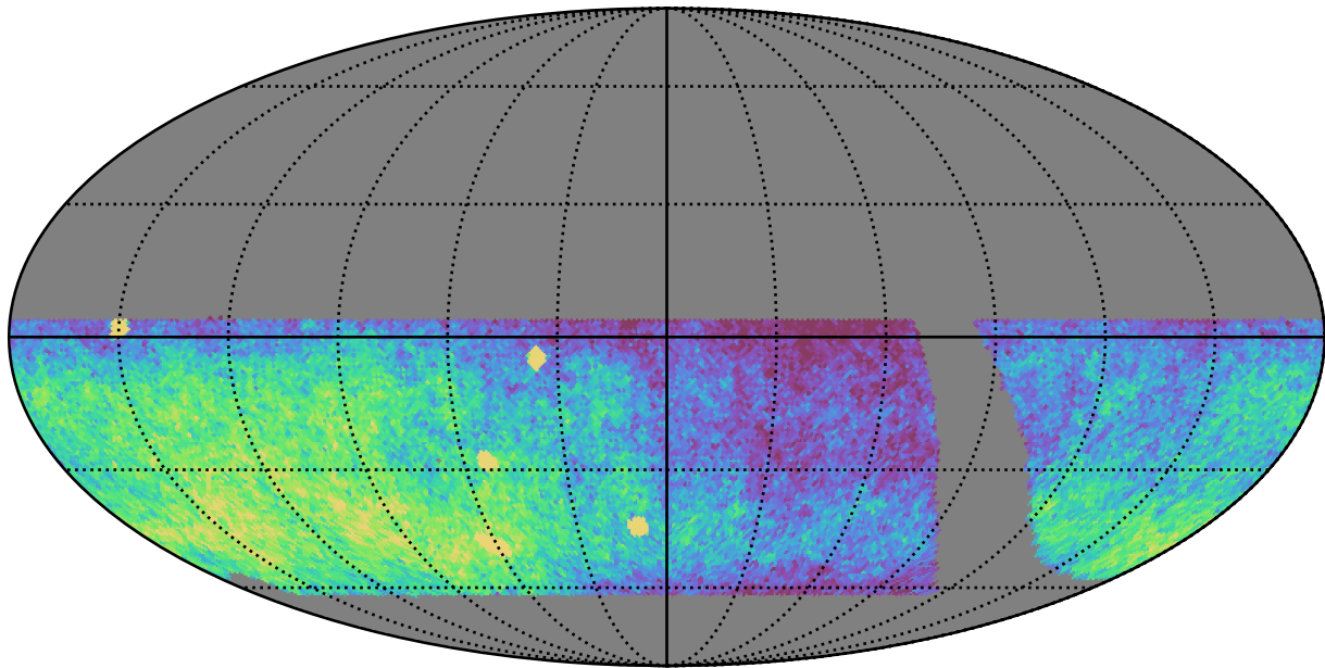
retro_baseline_v2.0_10yrs WFD g band: CoaddM5
