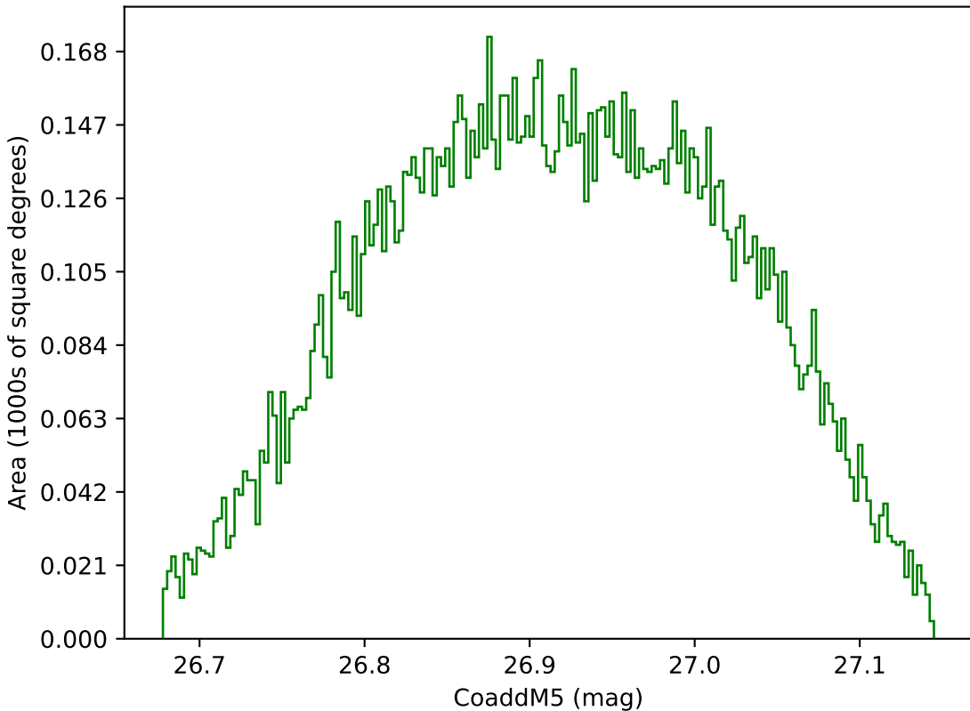
retro_baseline_v2.0_10yrs WFD g band: CoaddM5
