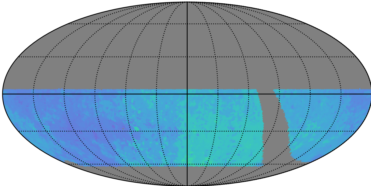
retro_baseline_v2.0_10yrs WFD z band: 80thPercentile Season Length
