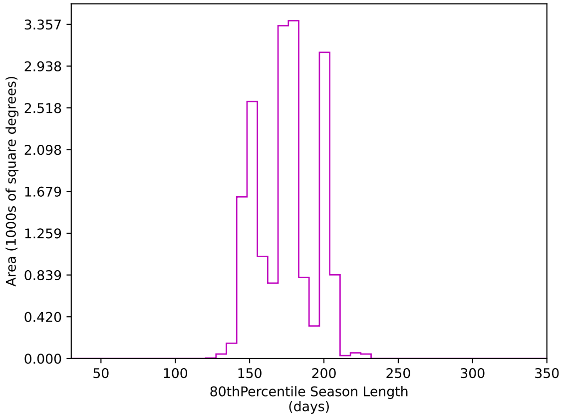
retro_baseline_v2.0_10yrs WFD z band: 80thPercentile Season Length
