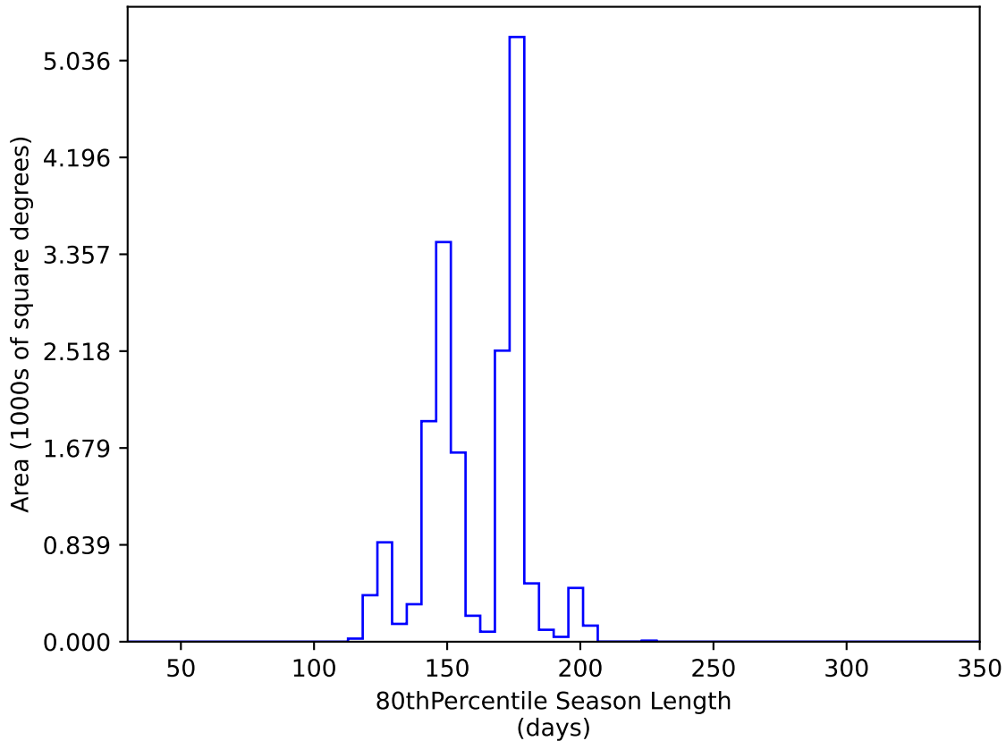
retro_baseline_v2.0_10yrs WFD y band: 80thPercentile Season Length
