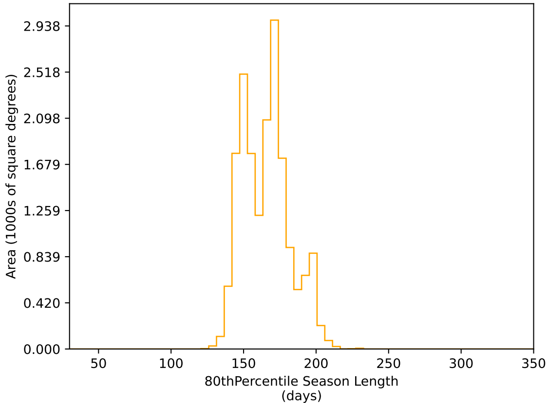
retro_baseline_v2.0_10yrs WFD r band: 80thPercentile Season Length
