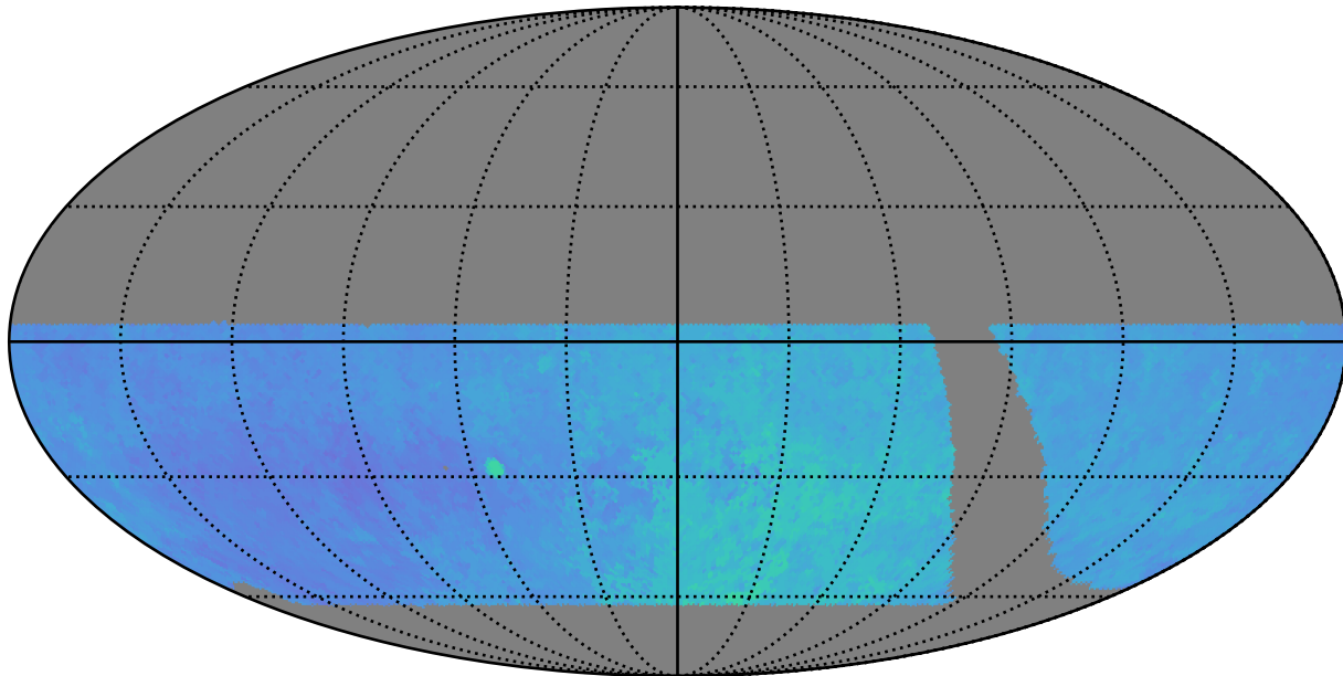
retro_baseline_v2.0_10yrs WFD i band: 80thPercentile Season Length
