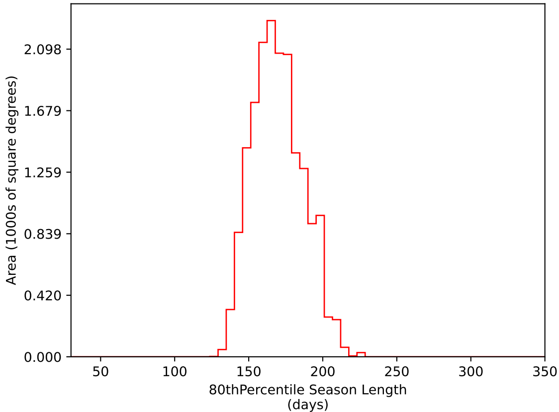
retro_baseline_v2.0_10yrs WFD i band: 80thPercentile Season Length
