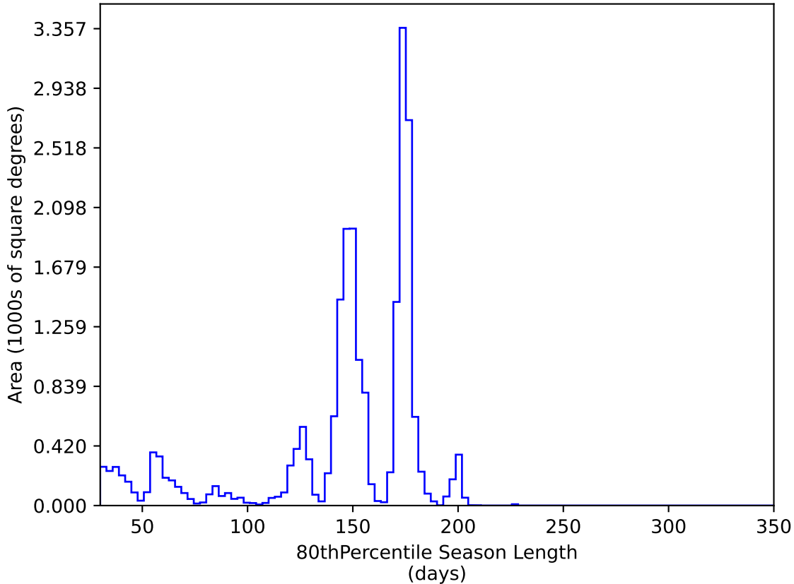
retro_baseline_v2.0_10yrs All sky y band: 80thPercentile Season Length
