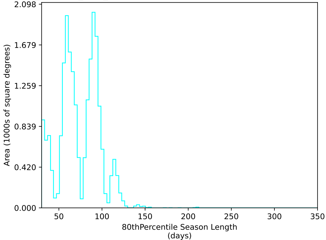
retro_baseline_v2.0_10yrs All sky u band: 80thPercentile Season Length
