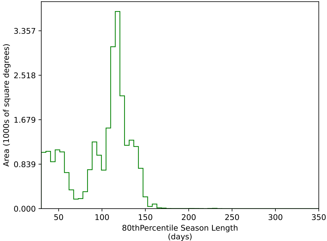
retro_baseline_v2.0_10yrs All sky g band: 80thPercentile Season Length
