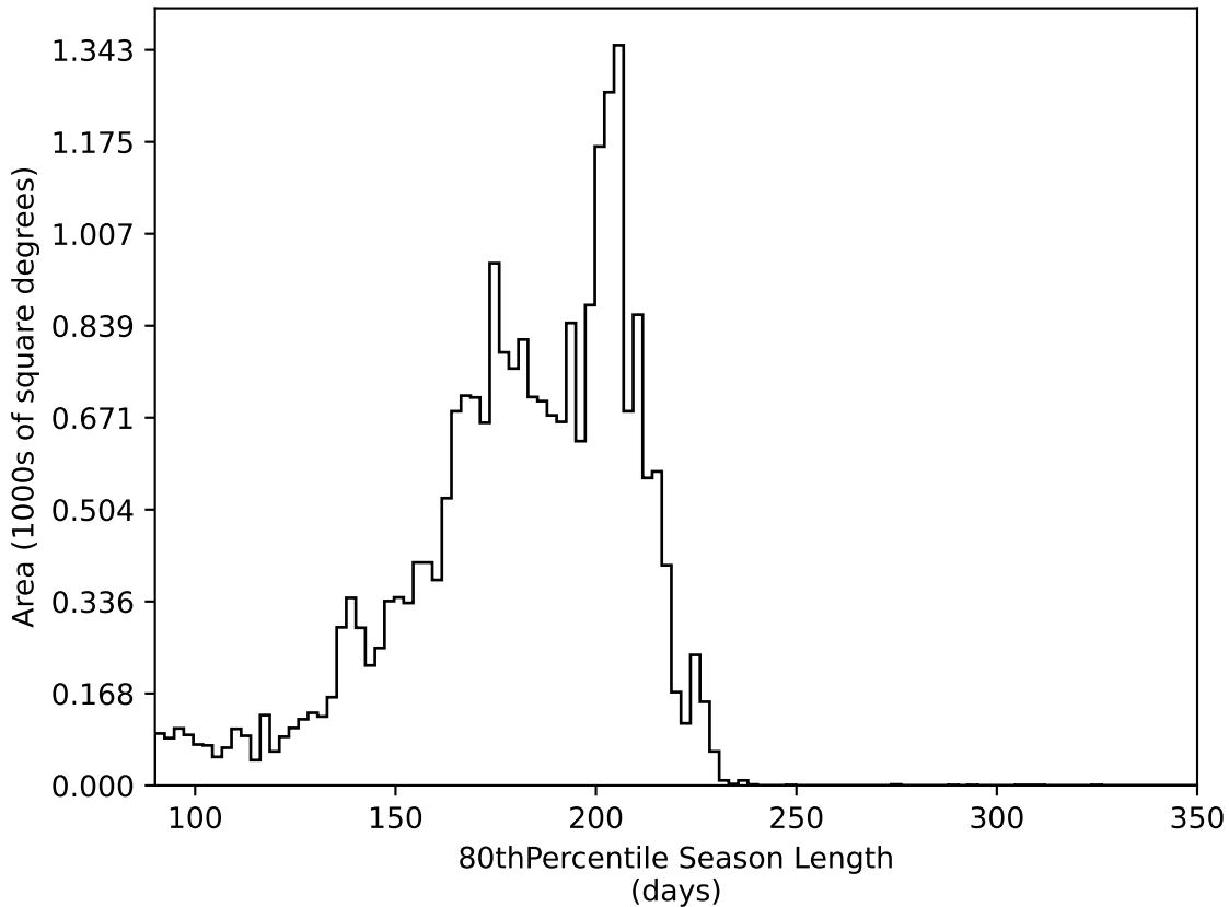
retro_baseline_v2.0_10yrs All sky all bands: 80thPercentile Season Length
