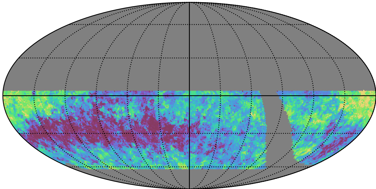
retro_baseline_v2.0_10yrs WFD zy bands: 75th Percentile Intranight Timespan
