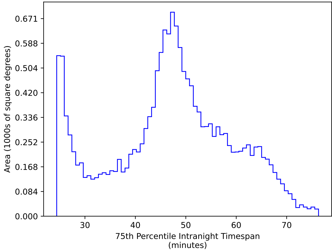
retro_baseline_v2.0_10yrs WFD zy bands: 75th Percentile Intranight Timespan
