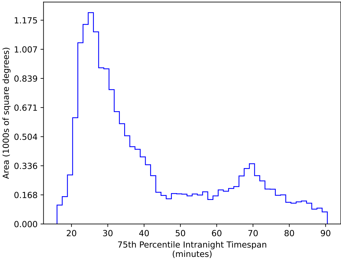
retro_baseline_v2.0_10yrs WFD z band: 75th Percentile Intranight Timespan
