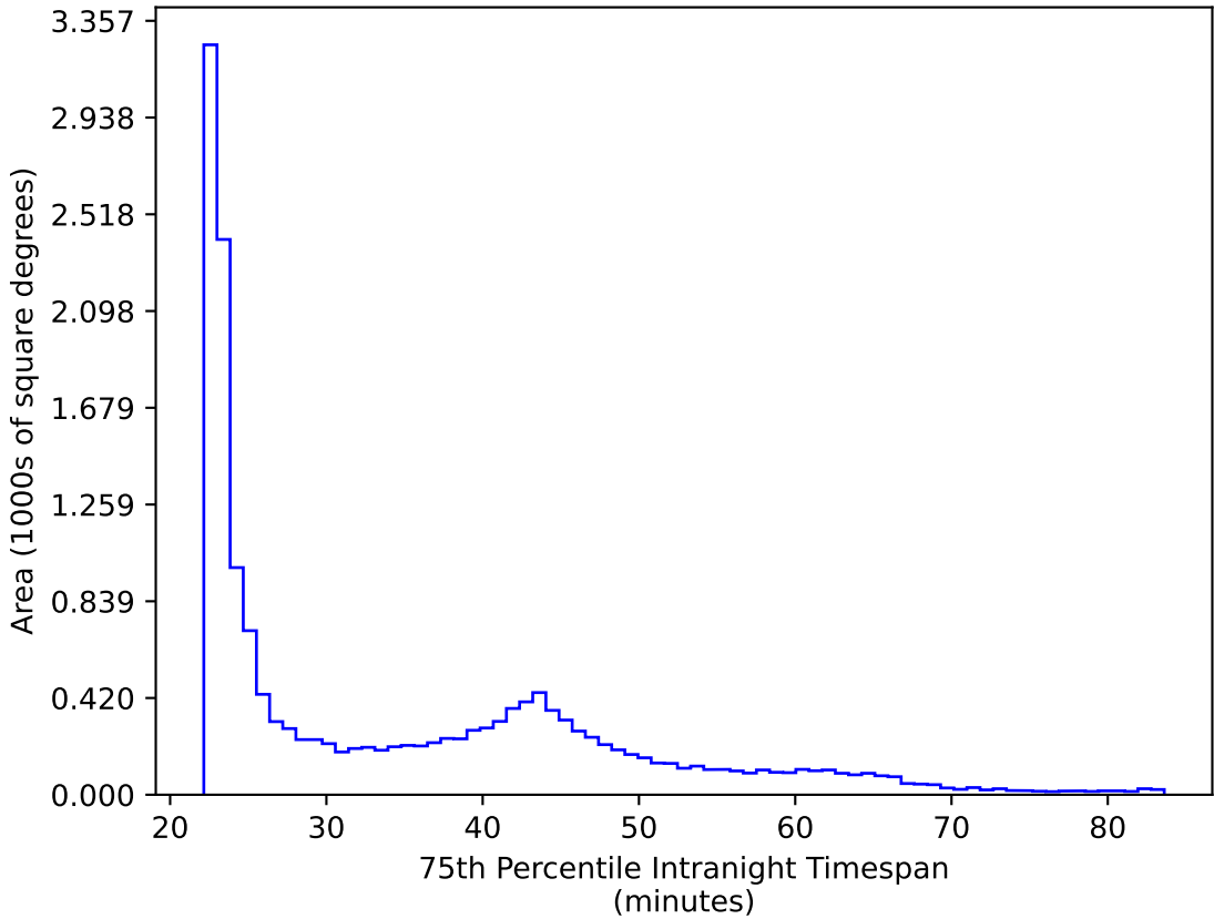
retro_baseline_v2.0_10yrs WFD y band: 75th Percentile Intranight Timespan
