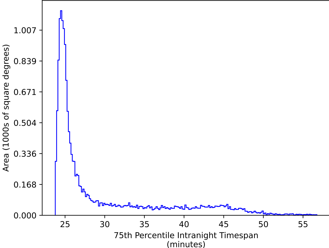
retro_baseline_v2.0_10yrs WFD ug bands: 75th Percentile Intranight Timespan
