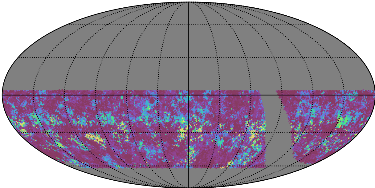
retro_baseline_v2.0_10yrs WFD u band: 75th Percentile Intranight Timespan
