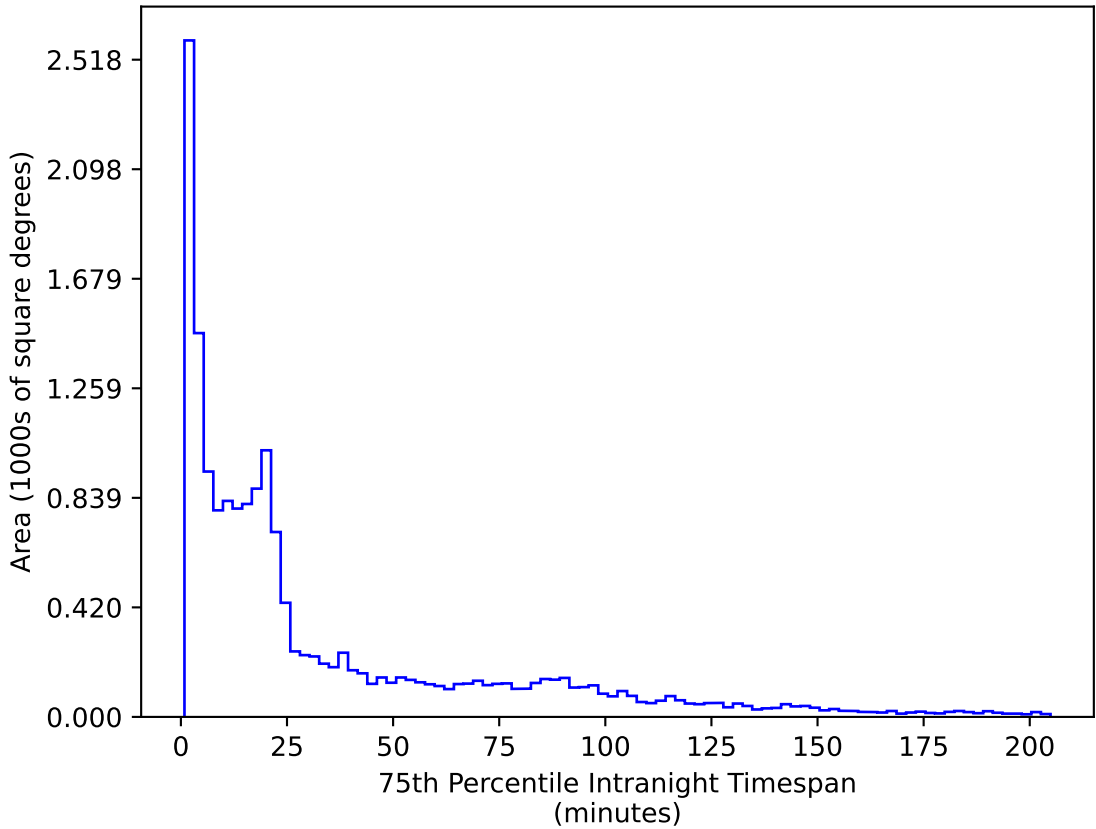
retro_baseline_v2.0_10yrs WFD u band: 75th Percentile Intranight Timespan
