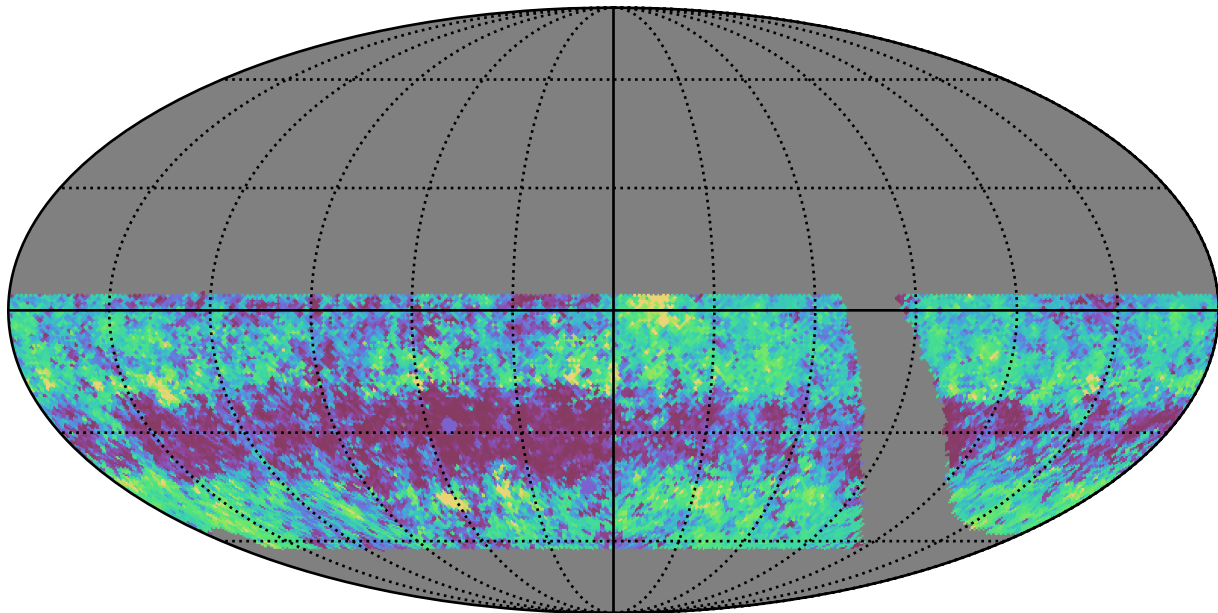
retro_baseline_v2.0_10yrs WFD ri bands: 75th Percentile Intranight Timespan
