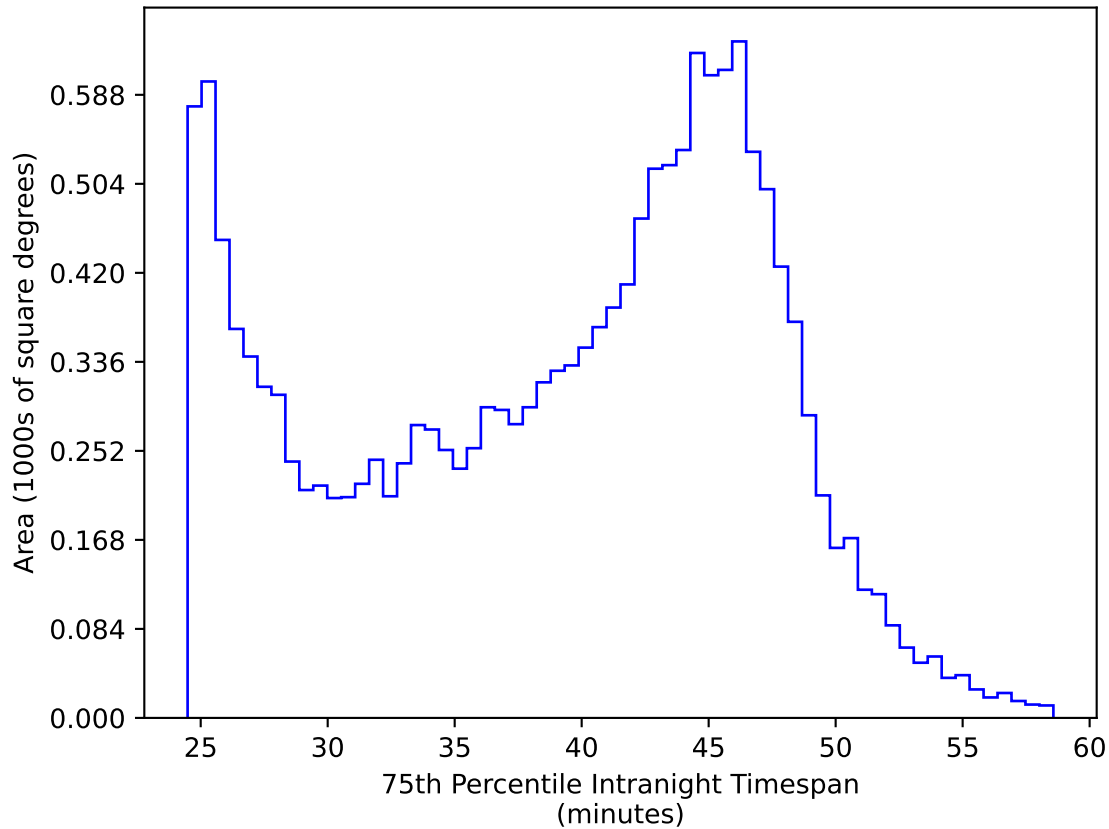
retro_baseline_v2.0_10yrs WFD ri bands: 75th Percentile Intranight Timespan
