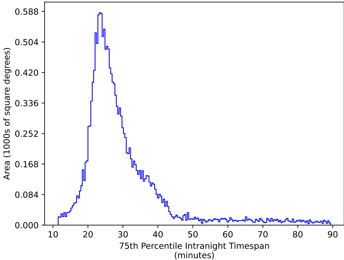
retro_baseline_v2.0_10yrs WFD r band: 75th Percentile Intranight Timespan
