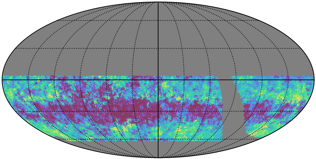
retro_baseline_v2.0_10yrs WFD gr bands: 75th Percentile Intranight Timespan
