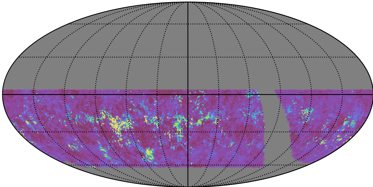
retro_baseline_v2.0_10yrs WFD g band: 75th Percentile Intranight Timespan
