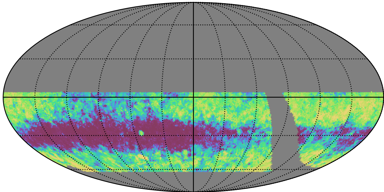
retro_baseline_v2.0_10yrs WFD all bands: 75th Percentile Intranight Timespan
