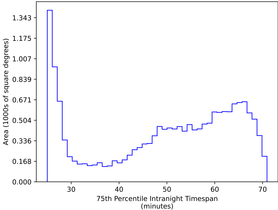
retro_baseline_v2.0_10yrs WFD all bands: 75th Percentile Intranight Timespan
