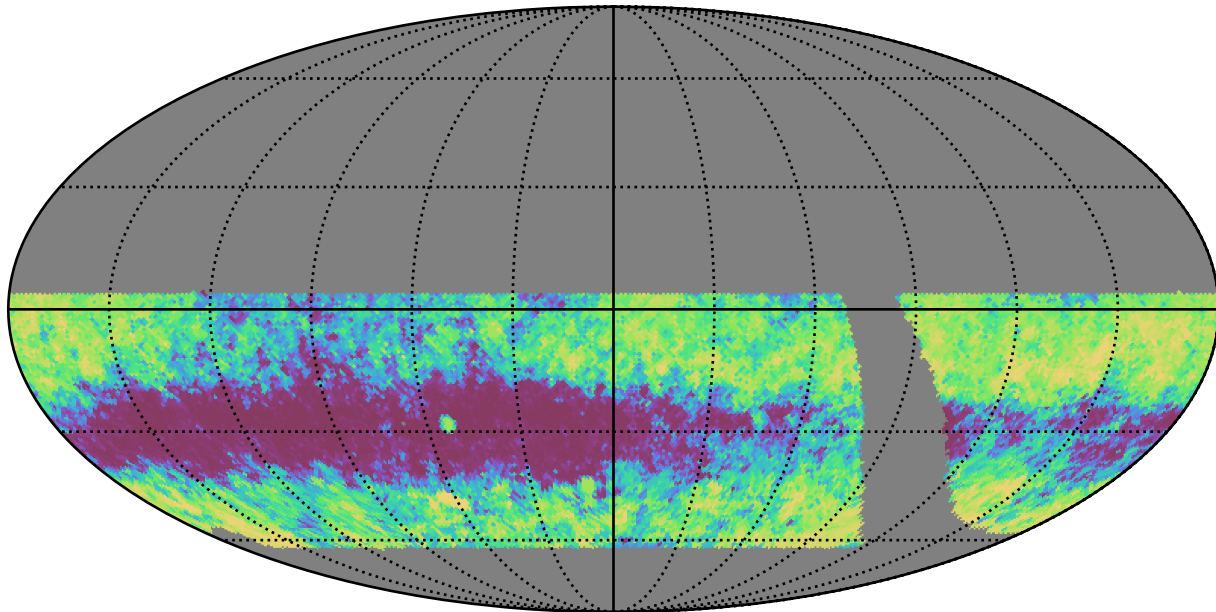
retro_baseline_v2.0_10yrs WFD: 75th Percentile Intranight Timespan
