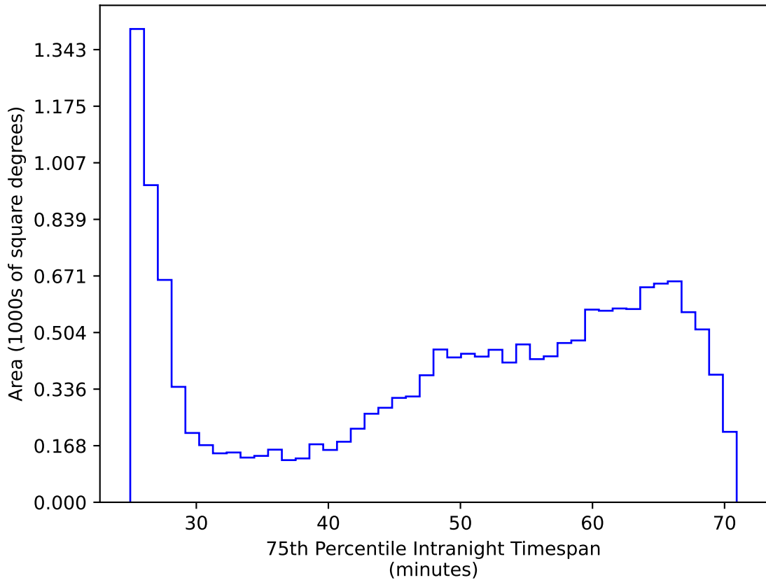
retro_baseline_v2.0_10yrs WFD: 75th Percentile Intranight Timespan
