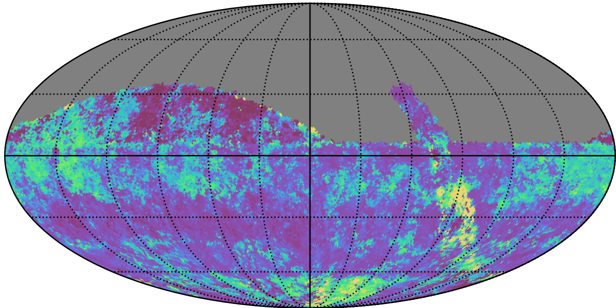
retro_baseline_v2.0_10yrs All sky z band: 75th Percentile Intranight Timespan
