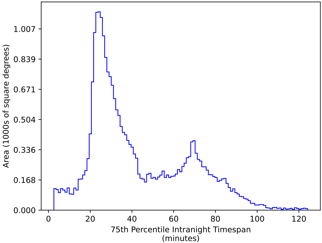
retro_baseline_v2.0_10yrs All sky z band: 75th Percentile Intranight Timespan
