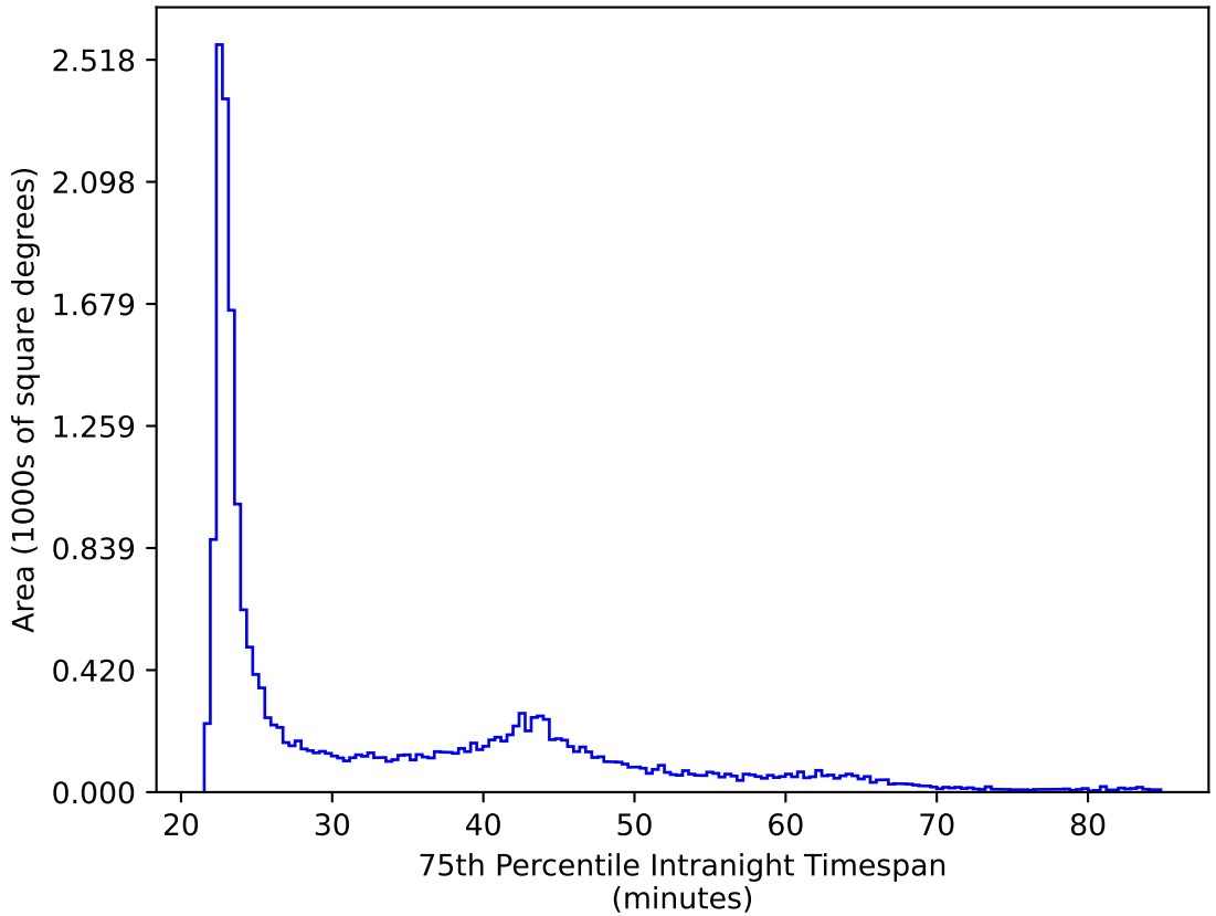
retro_baseline_v2.0_10yrs All sky y band: 75th Percentile Intranight Timespan
