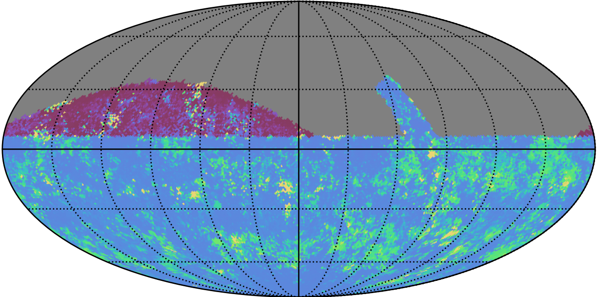
retro_baseline_v2.0_10yrs All sky ug bands: 75th Percentile Intranight Timespan
