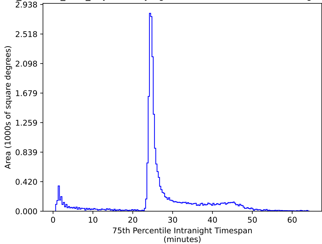
retro_baseline_v2.0_10yrs All sky ug bands: 75th Percentile Intranight Timespan
