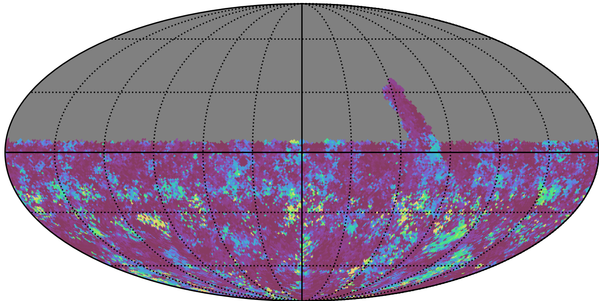
retro_baseline_v2.0_10yrs All sky u band: 75th Percentile Intranight Timespan
