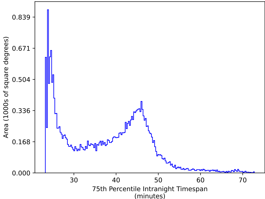
retro_baseline_v2.0_10yrs All sky ri bands: 75th Percentile Intranight Timespan
