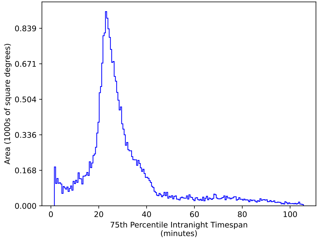
retro_baseline_v2.0_10yrs All sky r band: 75th Percentile Intranight Timespan
