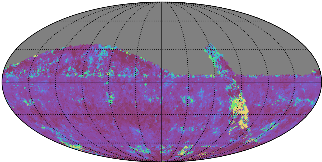
retro_baseline_v2.0_10yrs All sky i band: 75th Percentile Intranight Timespan
