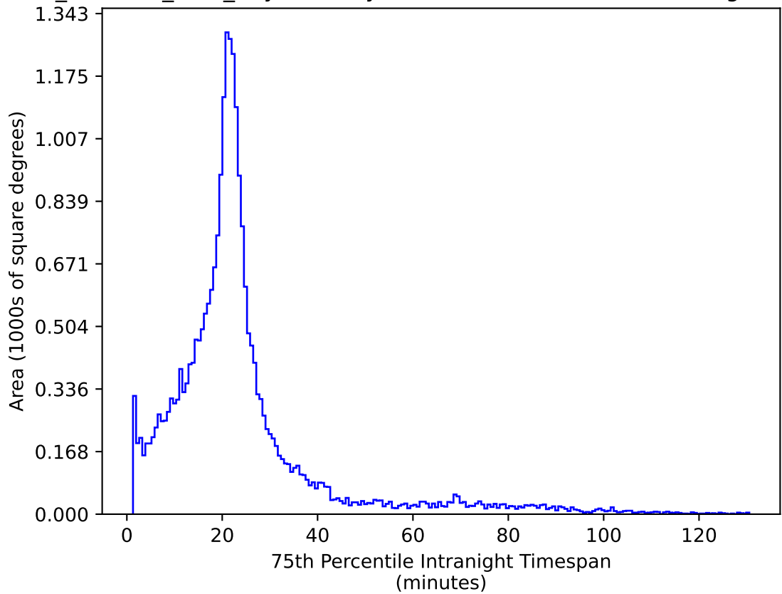
retro_baseline_v2.0_10yrs All sky i band: 75th Percentile Intranight Timespan
